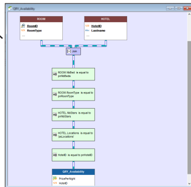
Embedded query: MyPage_1$Query
