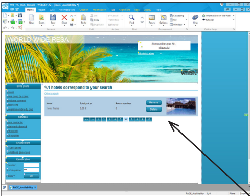
Looper linked to an embedded query
